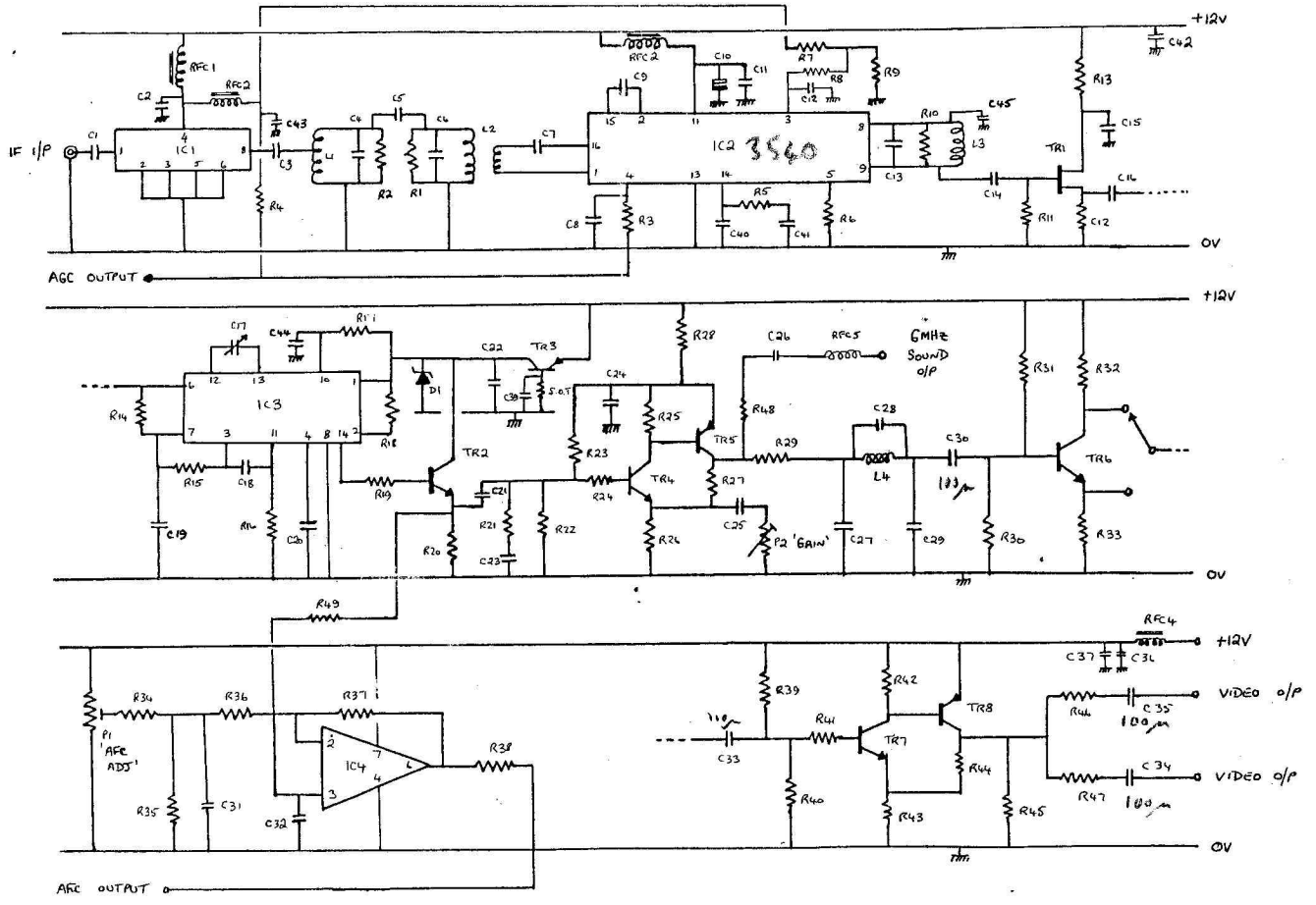
VIDIF CIRCUIT DIAGRAM
