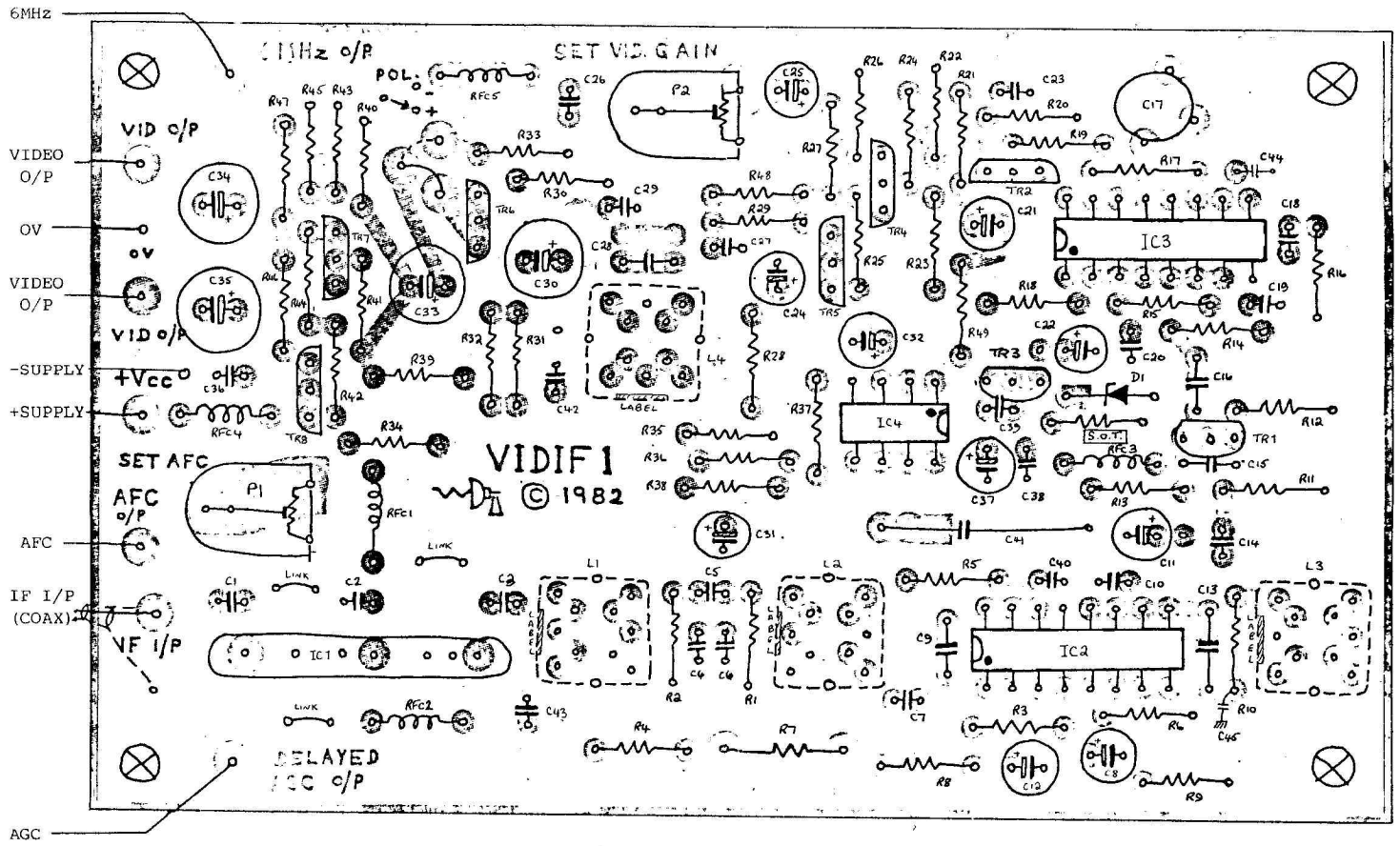
VIDIF Component Layout
