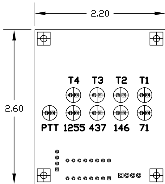
BOTTOM VIEW OF PCB PRINT USING 'Actual size'
