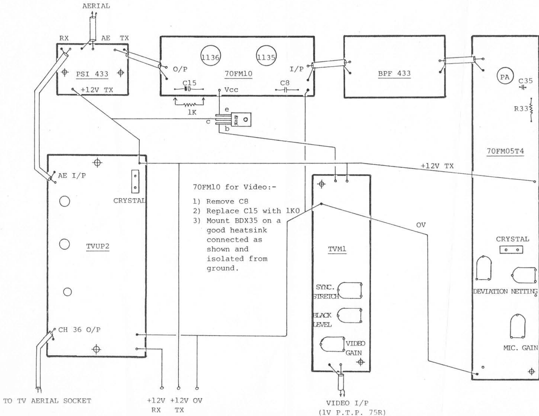
SYSTEM LAYOUT FULL LOW TV TRANSCEIVE PACKAGE
