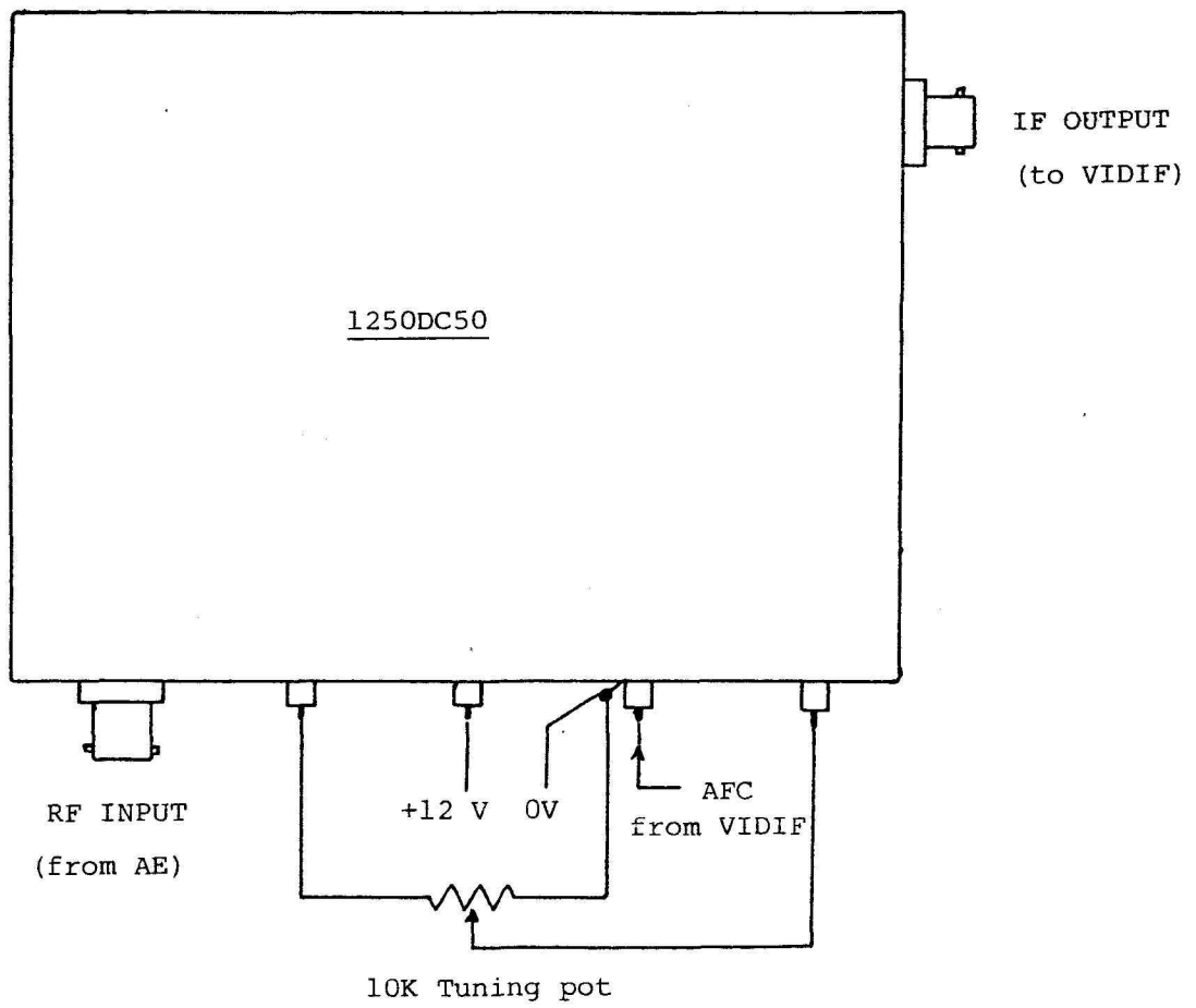
Connection Details for 1250DC50 Down Converter
